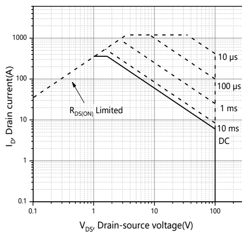
Figure 11. Safe operation area T C =25°C
